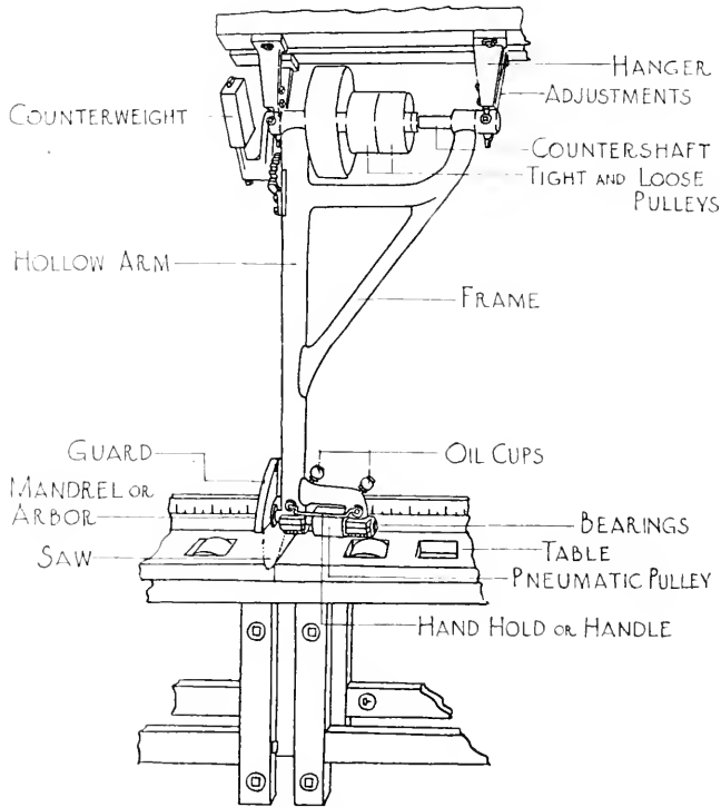
FIG. 133. SWING CUT-OFF SAW.
